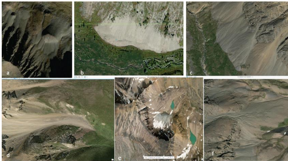
Figure 3: Landforms found in periglacial environments that can be considered embryonic rock glaciers (a) FOI; embryonic rock glacier (protalus lobe) from SA3, northern Mackenzie Mountains. ESRI world imagery base layer (EWIBL), 1:10,000 (b) protalus rampart, SA2,(EWIBL), 1:5,000; features that can be mistaken for rock glaciers (c) talus cones, SA1, ESRI World Imagery Base Layer, 1:5,000 (d) rockslide, SA2, ESRI (WIBL), 1:5,000 (e) debris covered glacier, SA1, ESRI (WIBL), 1:15,000 and (f) fluvial erosion over a talus slope, SA1, ESRI WIBL, 1:5,000. (ArcGIS Pro, version 2.9.3).
