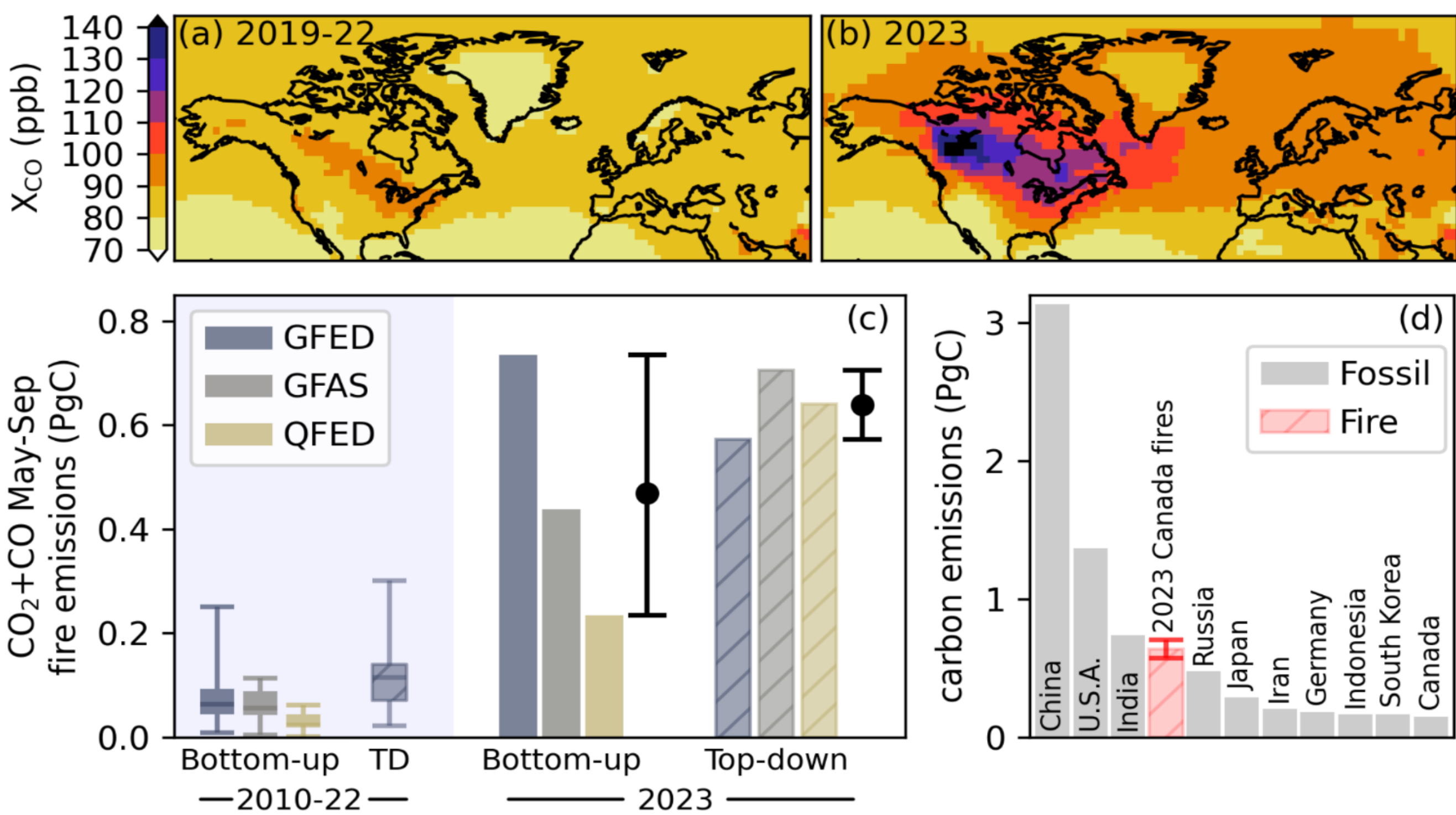
Fig.4. May-Sep TROPOMI XCO (a) averaged over 2019–2022 and (b) for 2023 aggregated to a 2° x 2.5° grid. (c) Canadian forest fire carbon emissions (from CO and CO2) for the 2023 May-Sep fire season, compared with fire emissions during 2010–2022 (distribution shown by box-and-whisker plots). Top-down emissions over 2010–2022 are estimated from MOPITT (2010–2021) and TROPOMI (2019–2022) CO retrievals. (d) A comparison of May-Sep Canadian fire emissions with 2022 territorial fossil carbon emissions for the 10 largest emitting countries, obtained from Global Carbon Budget 2022. These estimates are performed using three different prior bottom-up fire emission inventories: the Global Fire Emissions Database (GFED4.1s), the Global Fire Assimilation System version 1.2 (GFAS), and the Quick Fire Emissions Data set version 2.6r1 (QFED) inventories.
